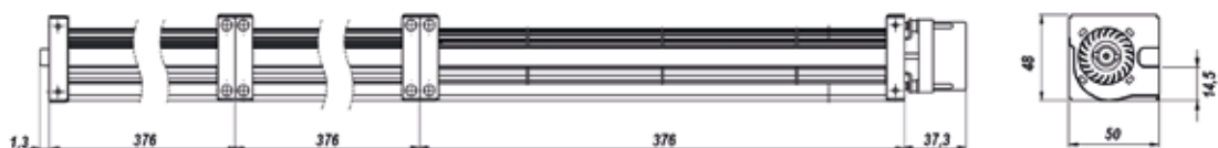
VTM-33-350-24DC-A-X
