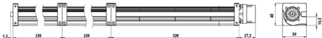
VTM-33-300-24DC-A-X
