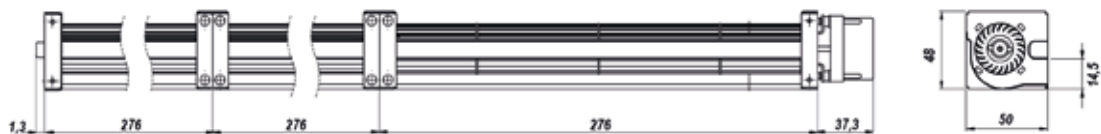
VTM-33-250-24DC-A-X
