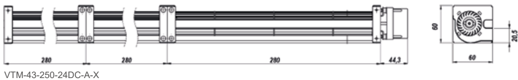
VTM-43-250-24DC-A-X
